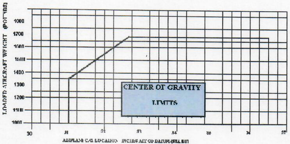
Figure 6-9 Center of Gravity Limits
