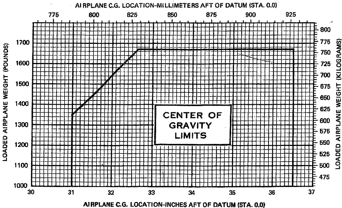
Figure 6-9. Center of Gravity Limits
